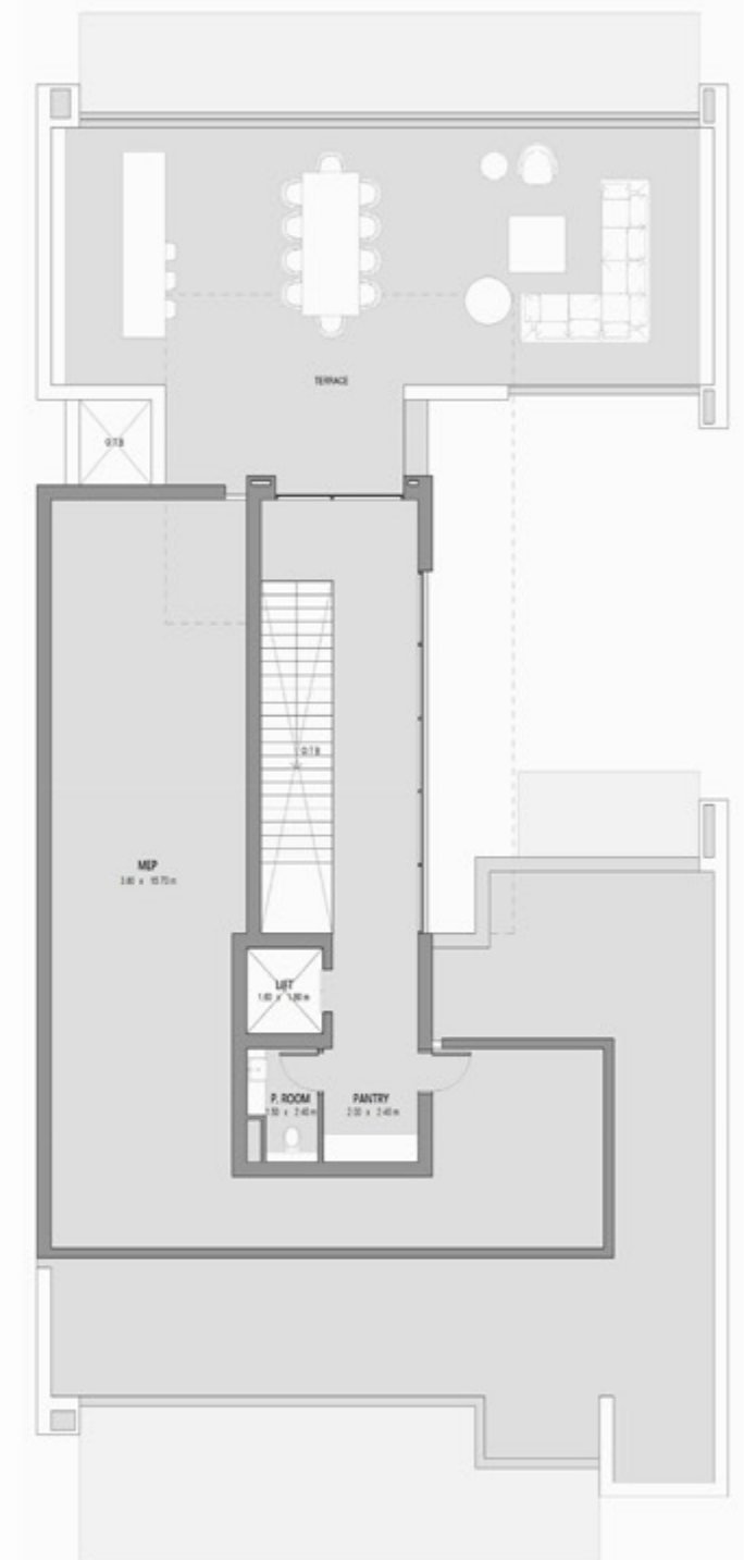
Roof Floor
